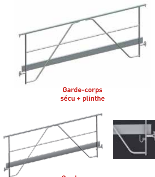
Garde-corps mds cat.2
